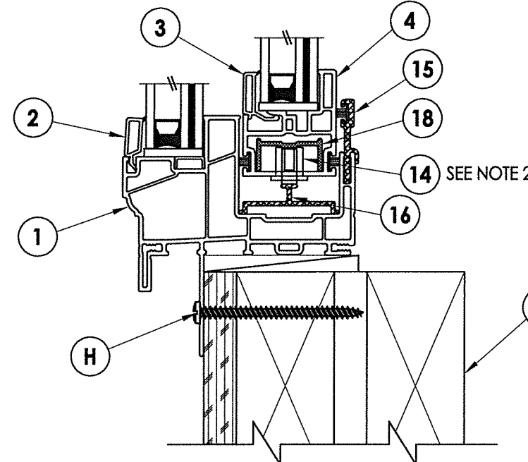
2 VERTICAL CROSS SECTION 3 2X Stud Construction
