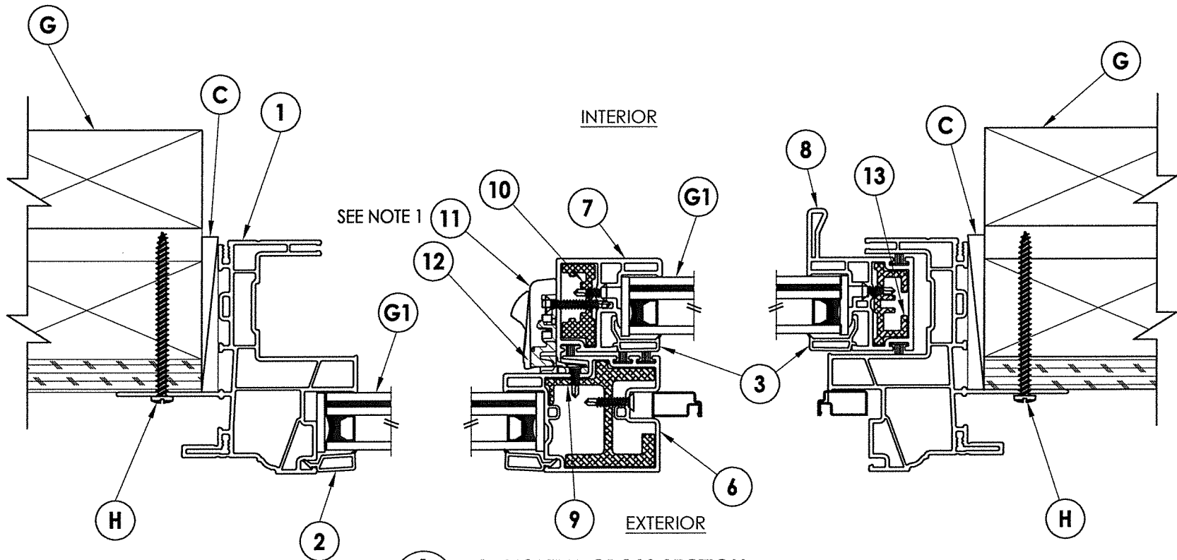
1 HORIZONTAL CROSS SECTION 3 2X Stud Construction
