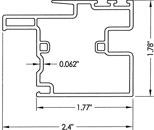
6 MEETING STILE
