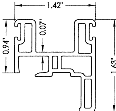
5 TOP RAIL
