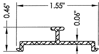
16 ROLLER TRACK
