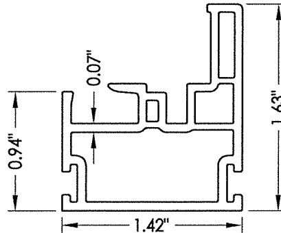
4 BOTTOM RAIL
