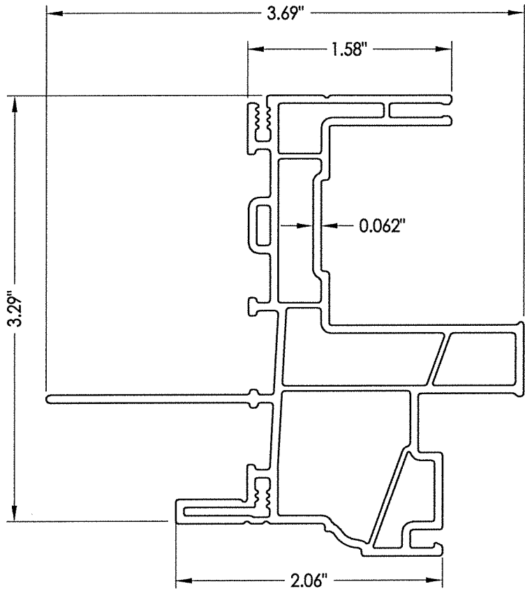
1 FRAME
