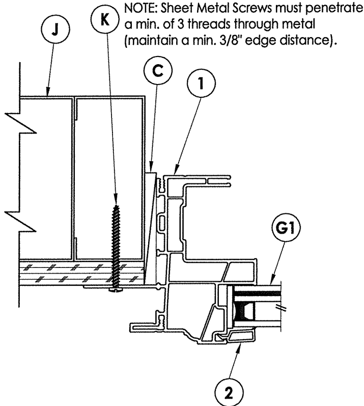
3 HORIZONTAL CROSS SECTION 3 Shown w/ Steel Stud Framing Option
